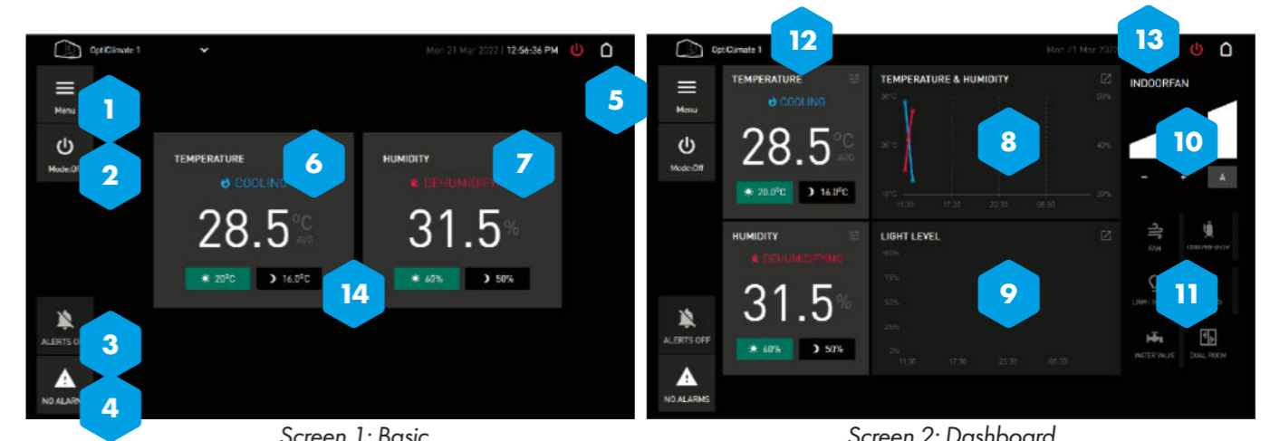
Screen 1: Basic
